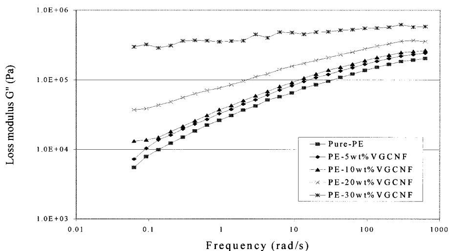
Figure 3 Loss modulus versus frequency at 190°C for the VGCNF-reinforced PE composites.
